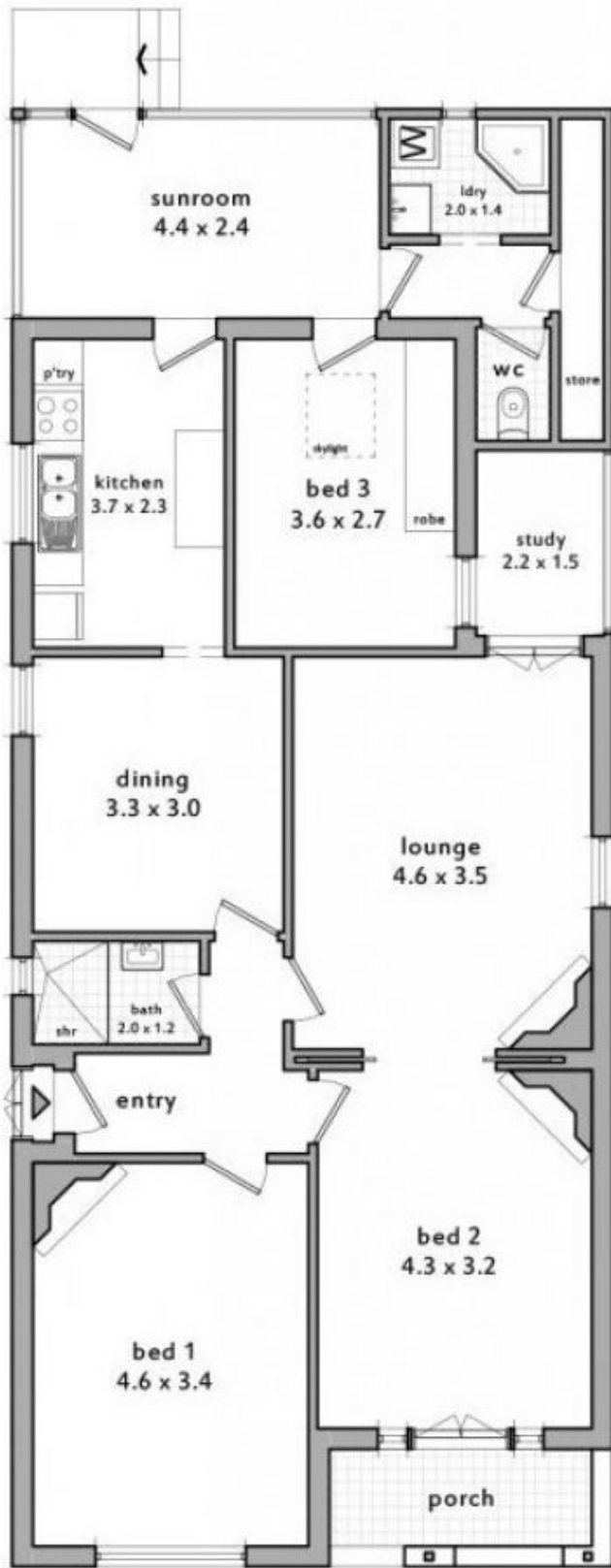
floor plan
